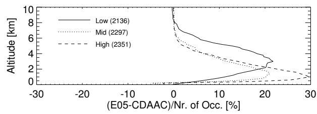
Figure 2. Relative difference of number of processed occultations over altitude for three latitude bands, # of matches in brackets.
