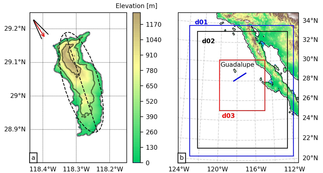
Figure 2. Topography of Guadalupe island. The Global Multi-resolution Terrain Elevation Data 2010 (GMTED2010) at 7.5 arc-seconds was used, and the dashed lines represent the fitted “mass density” ellipse and its major axis. The two black segments identify the range of the wind directions during the observed event, while the red arrow indicates the mean direction (panel a). The three nested domains used for the Weather Research and Forecasting simulations; the cross-section downstream the island was used for the Hövmoller diagrams (panel b).
