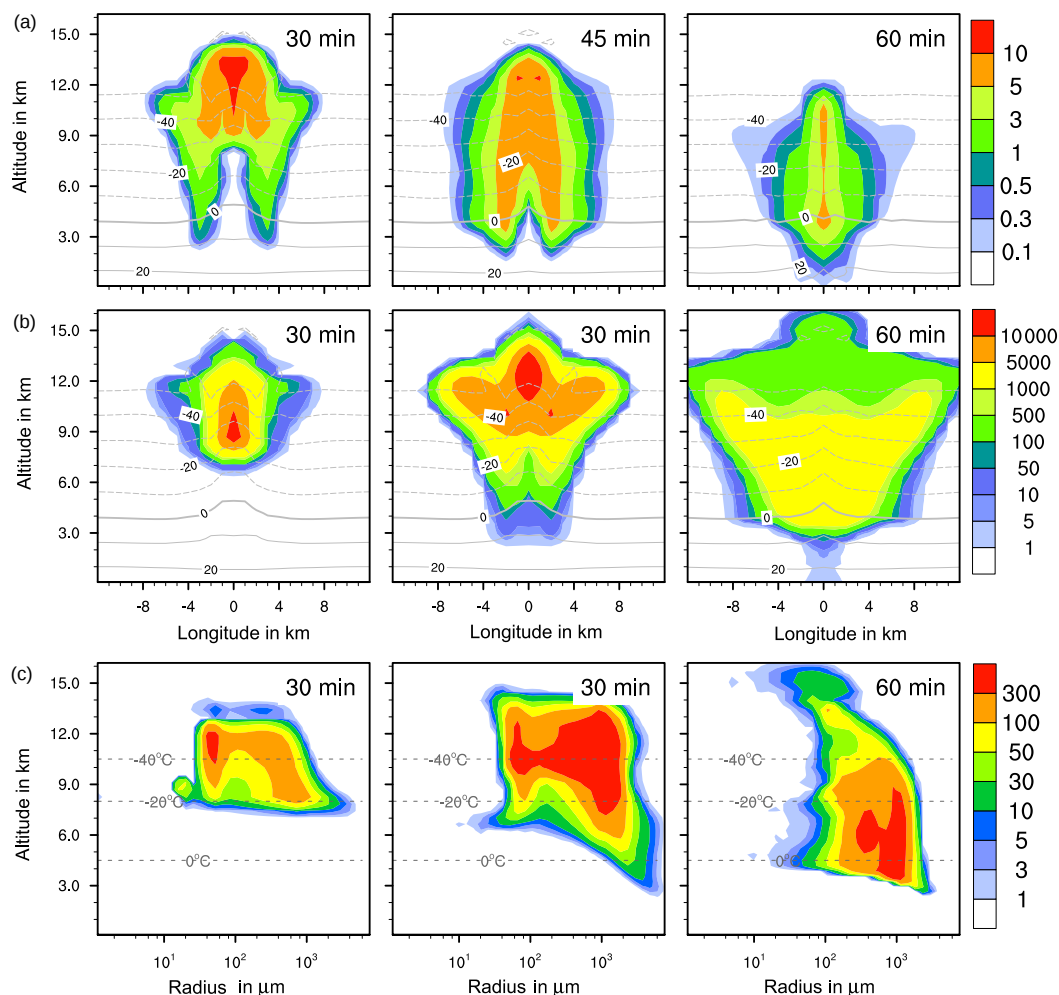
Figure 5. Ice formation from immersion freezing with 1 % feldspar. (a, b) Temporal development of two parameters shown in a vertical cut through the cloud center. Horizontal dashed lines: temperature in °C. (a) Ice water contents in \text{g kg}^{-1} and (b) ice particle numbers per \text{m}^3 . (c) Ice particle size spectra in the center cell of the cloud at different times. Number concentrations per \text{m}^3 . Left pictures in (b) and (c) show primary immersion freezing only.
