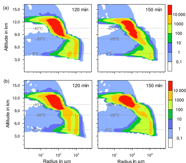
Figure 12. Ice particle size spectra in the center cell of the cloud after 120 and 150 min for cases with 1 % kaolinite–Saharan dust. Number concentrations per \text{m}^3 . (a) Solely immersion freezing and (b) combined immersion, deposition, and contact freezing.
