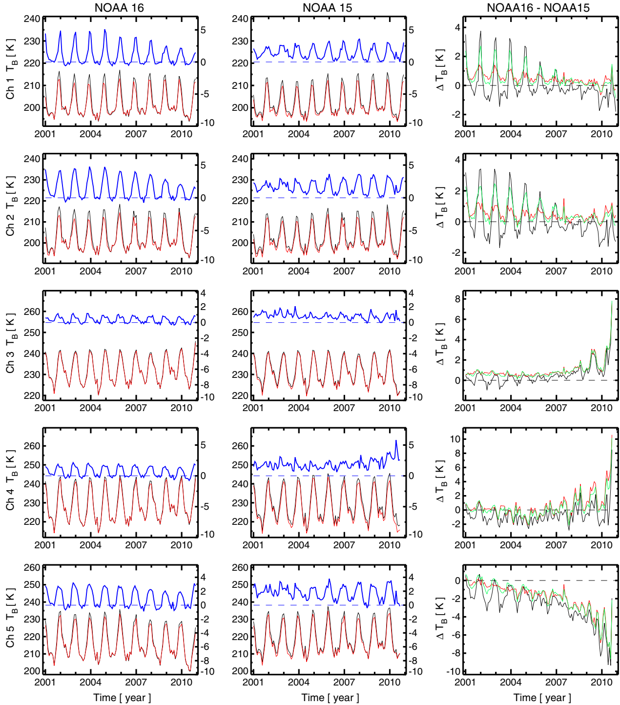
Figure 2. Monthly mean near-nadir brightness temperature for ascending (black) and descending (red) passes and their differences (blue; ascending minus descending) of (middle) NOAA 15 and (left) NOAA 16 from 2001 to 2010 over Antarctica ( 70^{\circ}\text{S} – 82^{\circ}\text{S} ). Right panels show intersatellite differences (N16–N15) for ascending passes (black), descending passes (red), and both combined (green).
