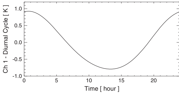
Figure 4. Diurnal cycle of Channel 1 brightness temperatures over tropical ocean. The method used to construct the diurnal cycle is described in Kottayil et al. [2013].
