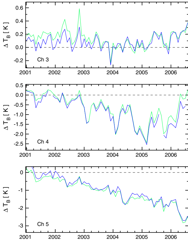
Figure 7. Intersatellite biases of Channels 3, 4, and 5 for N16 and N15 estimated using tropical ocean averages as described in section 3.1.2. Green curves represent bias estimates using all data and blue curves represent bias estimates using only cloud-unaffected data. Cloud filtering is based on Buehler et al. [2007].
