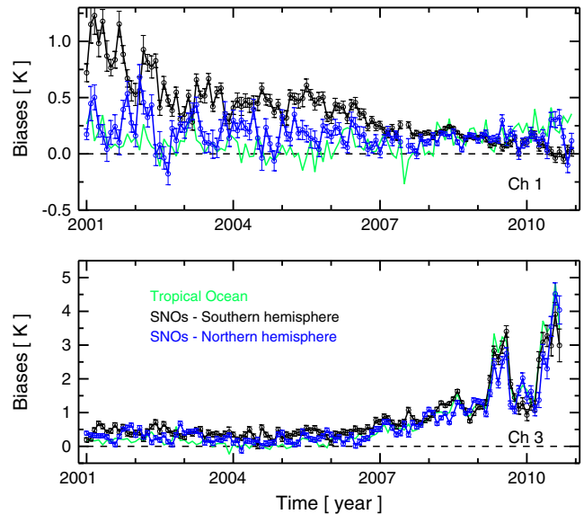
Figure 8. N16–N15 intersatellite bias estimates for Channels 1 and 3 using SNOs and tropical ocean measurements. SNO results from the two hemispheres are shown separately. Vertical bars for SNO bias estimates represent their standard error.
