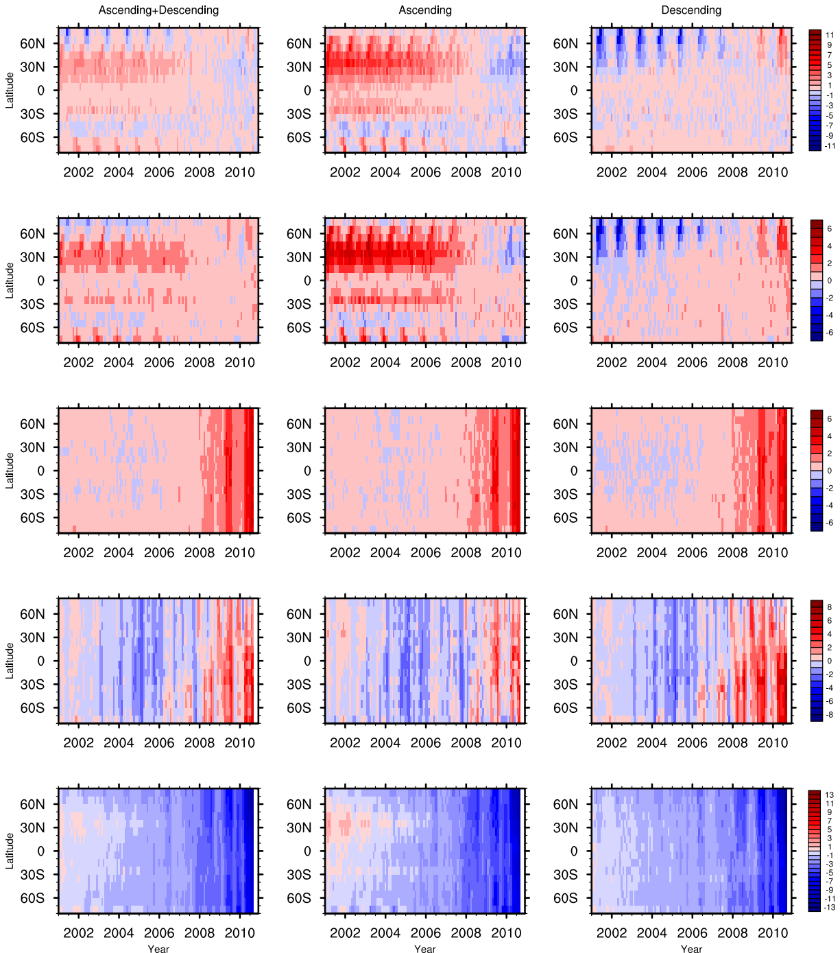
Figure 5. Biases (N16–N15, in kelvin) estimated from zonally averaged brightness temperatures for 16 latitude bands from 80°S to 80°N in 10° intervals are shown. Channel 1 is at first row, Channel 2 is at the second row, and so on. Left columns show biases estimated with data which consist of both ascending and descending passes. Middle columns are biases estimated with only ascending passes, and the right columns are biases estimated with only descending passes.
