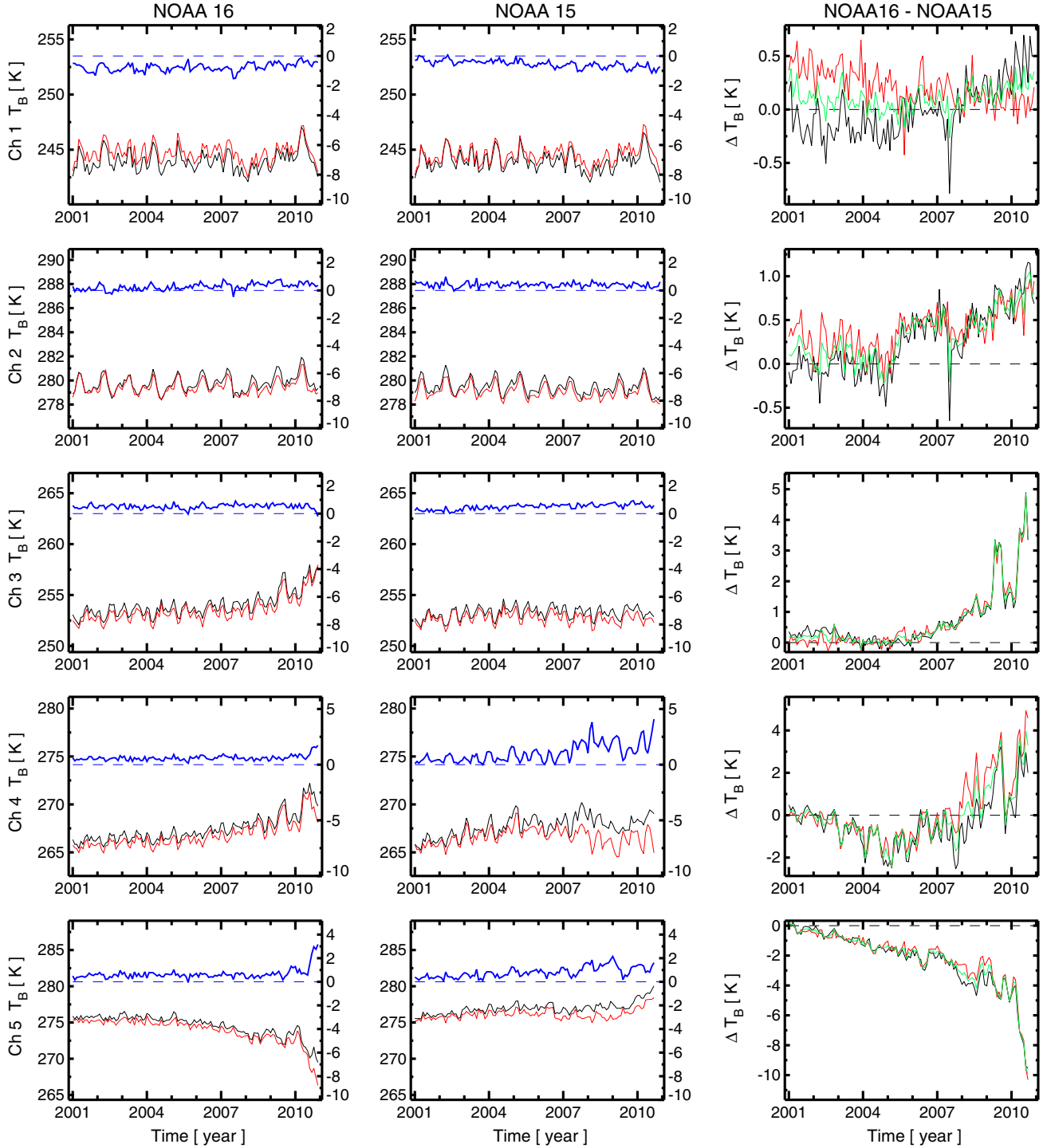
Figure 3. Monthly mean near-nadir brightness temperature for ascending (black) and descending (red) passes and their differences (blue; ascending minus descending) of (middle) NOAA 15 and (left) NOAA 16 from 2001 to 2010 over tropical oceans ( 20^{\circ}\text{S} – 20^{\circ}\text{N} ). Right panels show intersatellite differences (N16–N15) for ascending passes (black), descending passes (red), and both combined (green).
