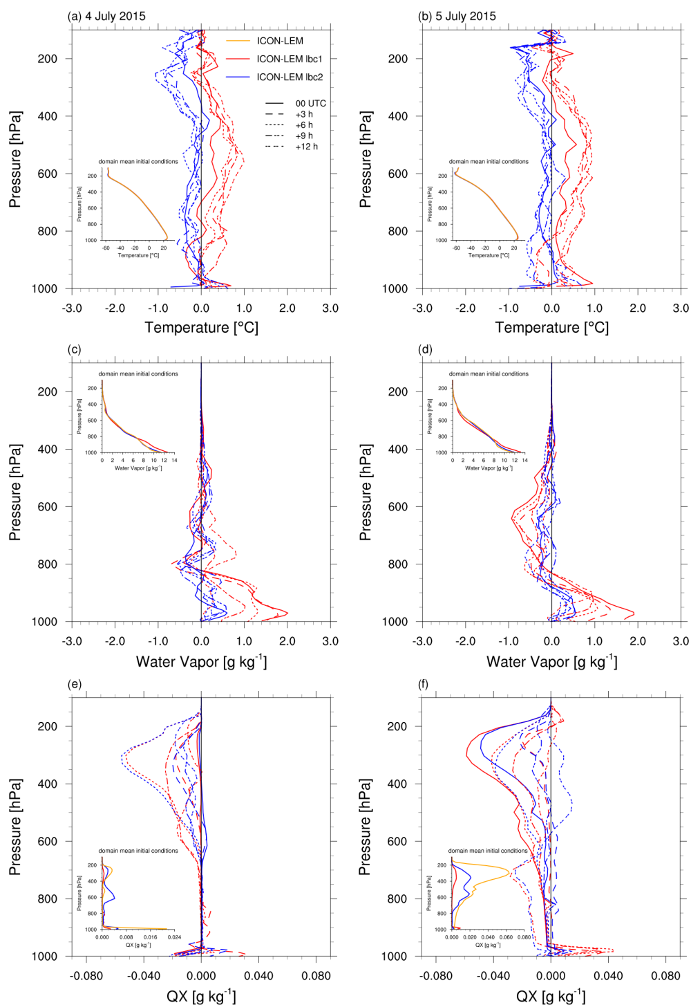
Figure A3. Initial and lateral boundary conditions used in Sect. 6.1 for temperature (a, b), water vapor (c, d), and total condensate, comprising cloud water, rain, ice, and snow (abbreviated as QX; e, f). The vertical profiles show differences using the ICON-NWP (ICON-LEM lbc1 – red) and IFS (ICON-LEM lbc2 – blue) analysis compared to the default simulation using analysis data provided by COSMO-DE. All forcing data sets are remapped onto the high-resolution ICON-LEM DOM01 grid. Solid lines (00:00 UTC) display a mean difference over the full domain, whereas the subsequent +3, +6, +9, and +12 h differences are averaged differences over the 20 km nudging zone at the domain edges, depicted with different line styles. The inlays show the mean initial (00:00 UTC) absolute profiles for the full domain including the control simulation (ICON-LEM – orange line). The vertical axes of the inlays are the same as in the difference plots. x axis labels span the temperature range between -60 and 10 °C; for water vapor the range is 0 to 14 g kg -1 and for condensate 0 to 0.024 g kg -1 .
