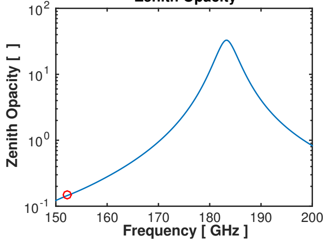
Zenith Opacity
