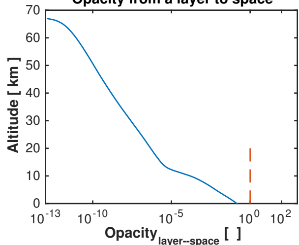
Opacity from a layer to space
