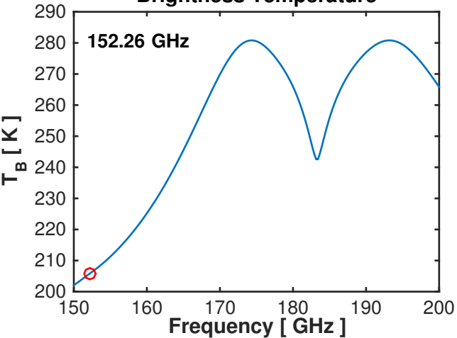
Brightness Temperature
