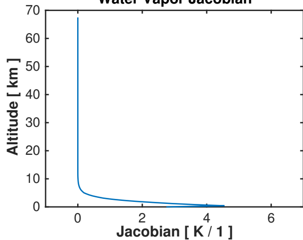
Water Vapor Jacobian
